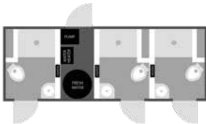
6x18' | 3-STATION, SHOWER COMBO FLOOR PLAN
