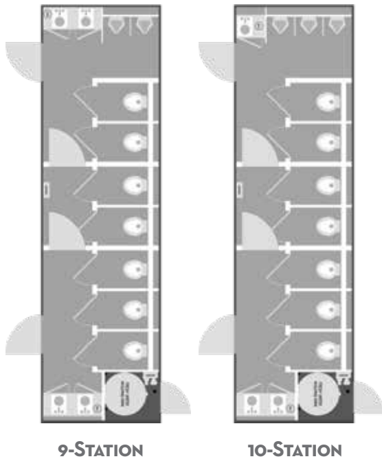
8x29' | FLEX FLOOR PLAN
