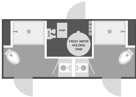
6x14' SHOWER COMBO FLOOR PLAN
