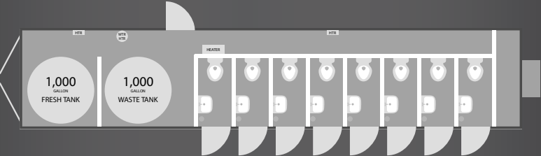
8x40' CUBE CONTAINER FLOOR PLAN
