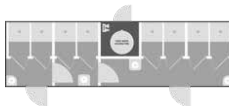
8x28' | 8-STATION, FLEX SHOWER FLOOR PLAN
