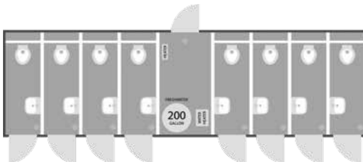
8x28' | 8-DOOR, 8-STATION FLOOR PLAN
