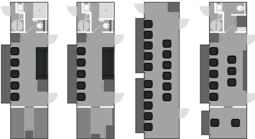
30' MULTI-PURPOSE WORKSTATION FLOOR PLANS
