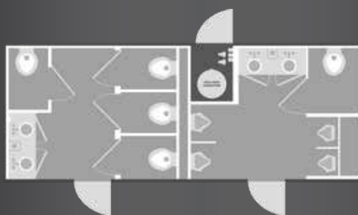
8x20' | 9-STATION FLOOR PLAN (OPTIONAL)
