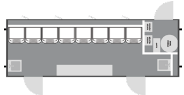
8x25' | 8-STATION, LAUNDRY FLOOR PLAN
