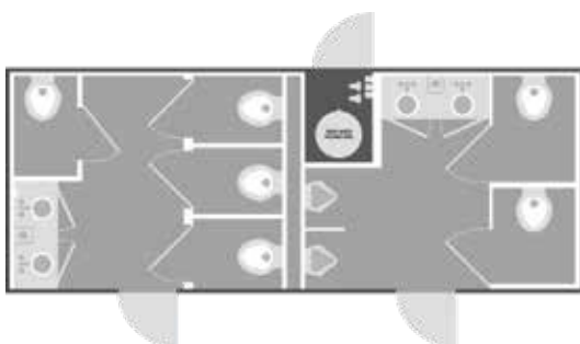
8x20' | 8-STATION FLOOR PLAN
