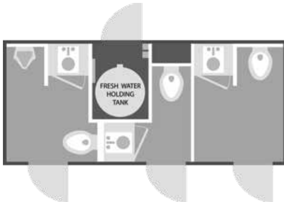
6x14' | 3-DOOR, 3-STATION FLOOR PLAN
