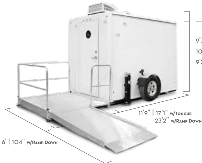
6'x11' | ADA, 1-STATION FLOOR PLAN
