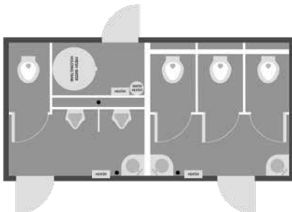
8x17' | 6-STATION FLOOR PLAN
