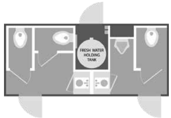
6x14' | 2-DOOR, 4-STATION FLOOR PLAN
